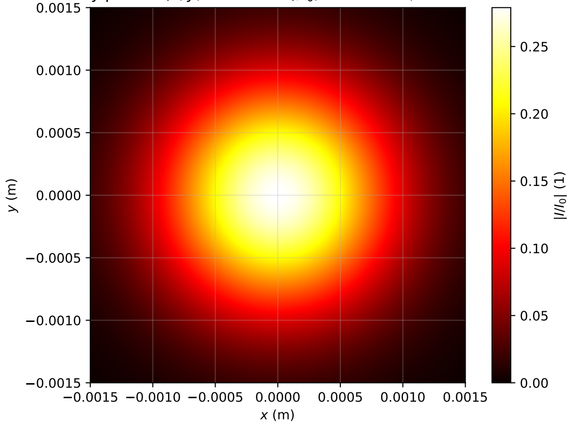
Intensity profile I(x, y, z = 3.423m)/I_0 , P_{in}=0.1P_{cr} , artificial time
